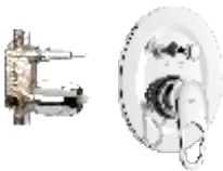
Single lever concealed diverter system consisting of Exposed part (lever, tip ton knob, flange) and Concealed part (40 mm cartridge with button assembly, cartridge sleeve) Exposed part F1002701 ₹ 1800 Concealed part F4010101 ₹ 3045 Set ₹ 4845
