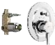
Single lever concealed diverter system consisting of Exposed part (lever, tip ton knob, wall flange) and Concealed part (40 mm cartridge with button assembly, cartridge sleeve) Exposed part F1017701 ₹ 1650 Concealed Part F4010101 ₹ 3045 Set ₹ 4695
