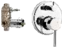
Turn type single lever concealed diverter system consisting of Exposed part (lever, tip ton knob, flange) and Concealed part (40 mm cartridge with button assembly, cartridge sleeve) Exposed part F2004703 ₹ 1805 Concealed part F4010105 ₹ 3350 Set ₹ 5155
