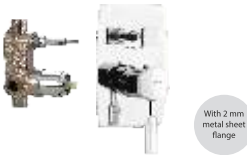
Single lever concealed diverter system consisting of Exposed part (lever, tip ton knob, 2 mm sheet flange) and Concealed part (35 mm cartridge with button assembly, cartridge sleeve) Exposed part F1014702 ₹ 1640 Concealed Part F4010103 ₹ 2795 Set ₹ 4435
