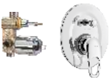
High flow single lever concealed diverter system consisting of Exposed part (lever, tip ton knob, flange) and Concealed part (45 mm cartridge with button assembly, cartridge sleeve) Exposed part F1002721 ₹ 2105 Concealed part F4030101 ₹ 3880 Set ₹ 5985
