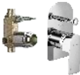
Single lever concealed diverter system consisting of Exposed part (lever, tip ton knob, flange) and Concealed part (40 mm cartridge with button assembly, cartridge sleeve) Exposed part F1016701 ₹ 2160 Concealed Part F4010101 ₹ 3045 Set ₹ 5205
