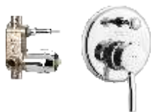
Single lever concealed diverter system consisting of Exposed part (lever, tip ton knob, flange) and Concealed part (40 mm cartridge with button assembly, cartridge sleeve)
