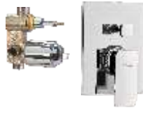
High flow single lever concealed diverter system consisting of Exposed part (lever, tip ton knob, flange) and Concealed part (45 mm cartridge with button assembly, cartridge sleeve) Exposed part F1005721 ₹ 2500 Concealed part F4030101 ₹ 3880 Set ₹ 6380
