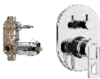
Turn type single lever concealed diverter system consisting of Exposed part (lever, turn type knob, flange) and Concealed part (40 mm cartridge with button assembly, cartridge sleeve) Exposed part F1007703 ₹ 1925 Concealed part F4010105 ₹ 3350 Set ₹ 5275
