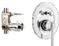
Single lever concealed diverter system consisting of Exposed part (lever, tip ton knob, flange) and Concealed part (40 mm cartridge with button assembly, cartridge sleeve) Exposed part F2003701 ₹ 1640 Concealed part F4010101 ₹ 3045 Set ₹ 4685
