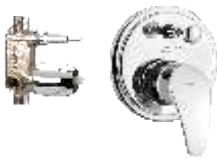
Single lever concealed diverter system consisting of Exposed part (lever, tip ton knob, flange) and Concealed part (40 mm cartridge with button assembly, cartridge sleeve) Exposed part F1001701 ₹ 1840 Concealed part F4010101 ₹ 3045 Set ₹ 4885
