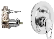
5-way (3 inlets + 2 outlets) single lever concealed diverter system consisting of Exposed part (lever, tip ton knob, flange) and Concealed part (cartridge with button assembly, cartridge sleeve) Exposed part F1002711 ₹ 2000 Concealed part F4020101 ₹ 3755 Set ₹ 5755
