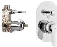
5-way (3 inlets + 2 outlets) single lever concealed diverter system consisting of Exposed part (lever, tip ton knob, flange) and Concealed part (cartridge with button assembly, cartridge sleeve) Exposed part F1018711 ₹ 2380 Concealed Part F4020101 ₹ 3755 Set ₹ 6135
